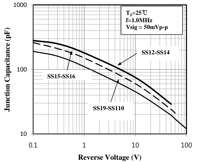
Fig.6 Typical Capacitance
