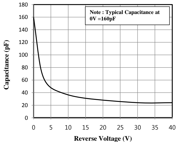
Fig.6 Typical Capacitance
